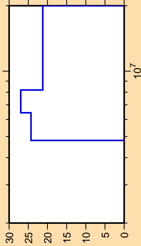
\Delta\sigma/\sigma vs. E for ^{186}\text{Ta}(n,n_1)
