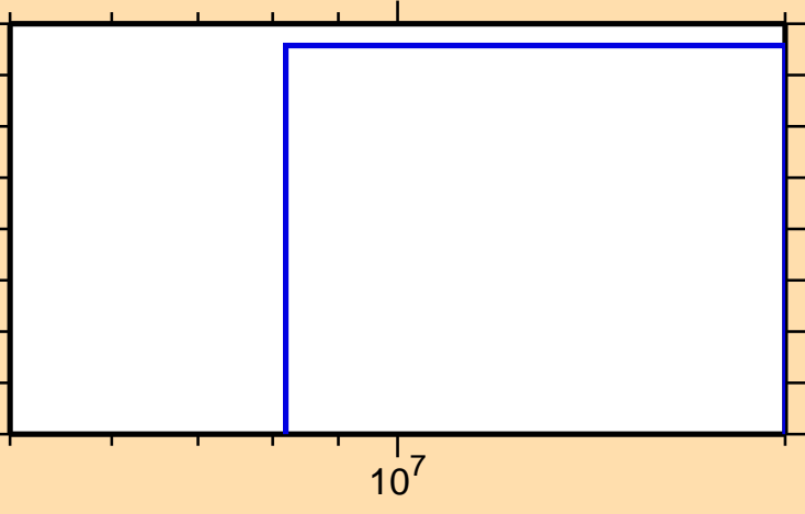
\sigma vs. E for ^{186}\text{Ta}(n,d)
