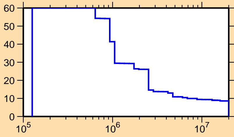
\Delta\sigma/\sigma vs. E for ^{187}\text{Ta}(n,\text{nonel.})
