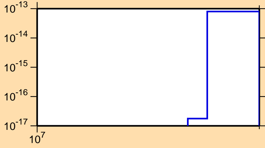
\sigma vs. E for ^{187}\text{Ta}(n,3n\alpha)
