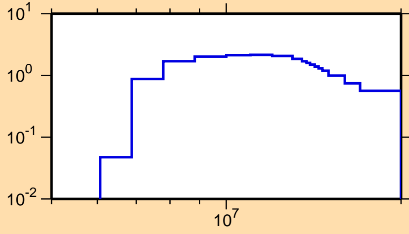
\sigma vs. E for ^{187}\text{Ta}(n,2n)
