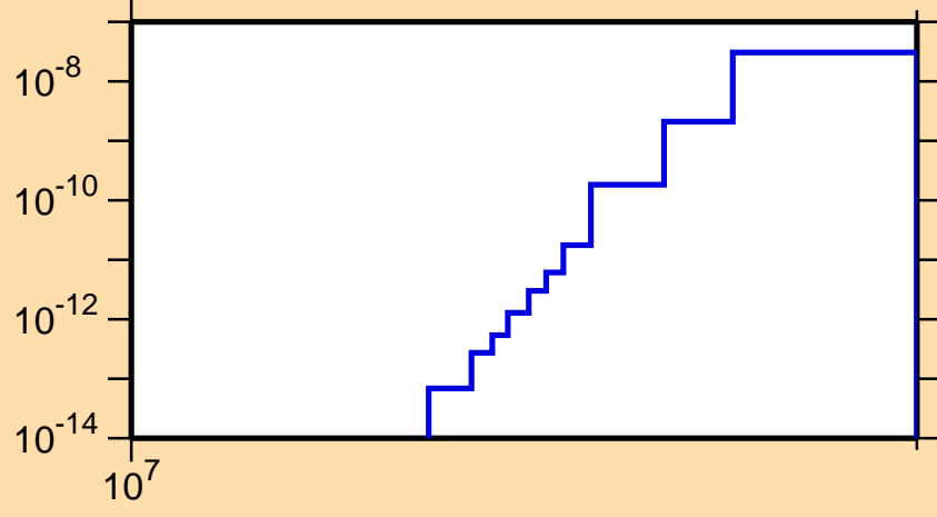
\sigma vs. E for ^{187}\text{Ta}(n,2n\alpha)
