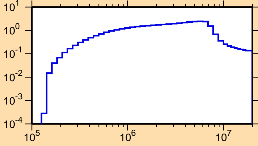
\sigma vs. E for ^{187}\text{Ta}(n,n\text{cont.})
