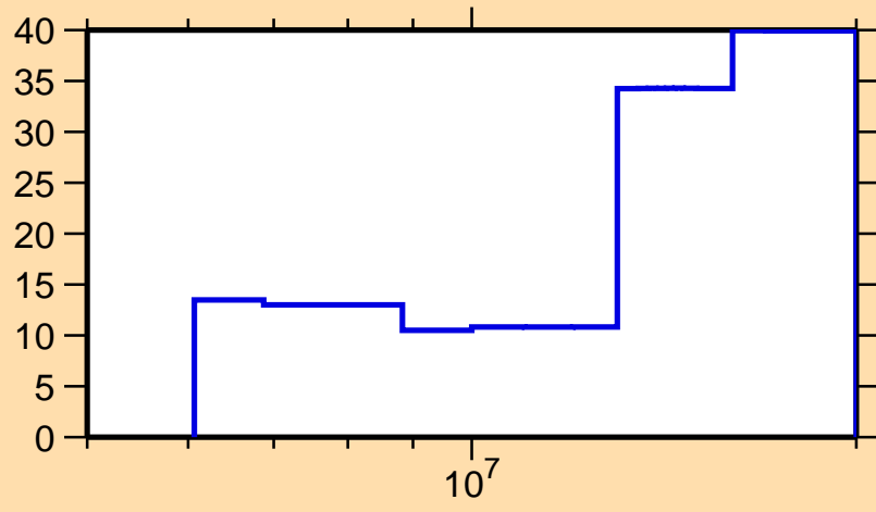
\Delta\sigma/\sigma vs. E for ^{187}\text{Ta}(n,2n)
