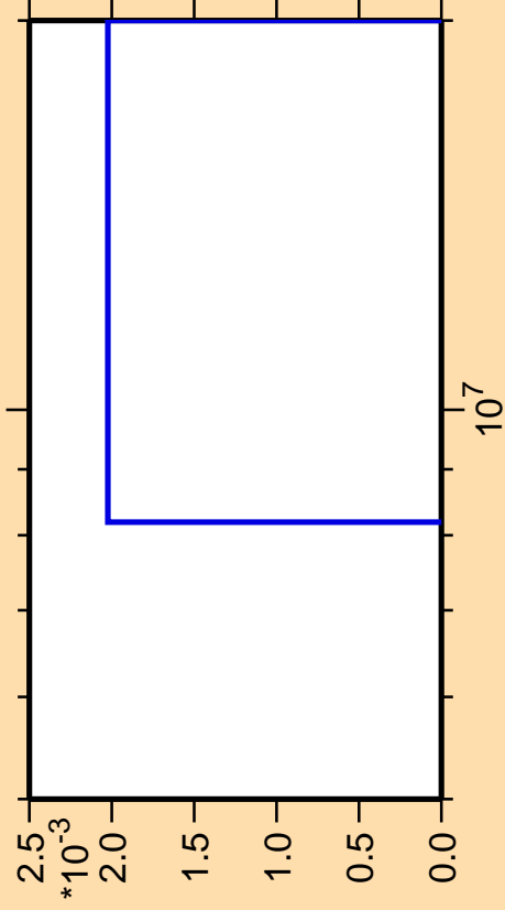
\Delta\sigma/\sigma vs. E for ^{187}\text{Ta}(n,3n\alpha)
