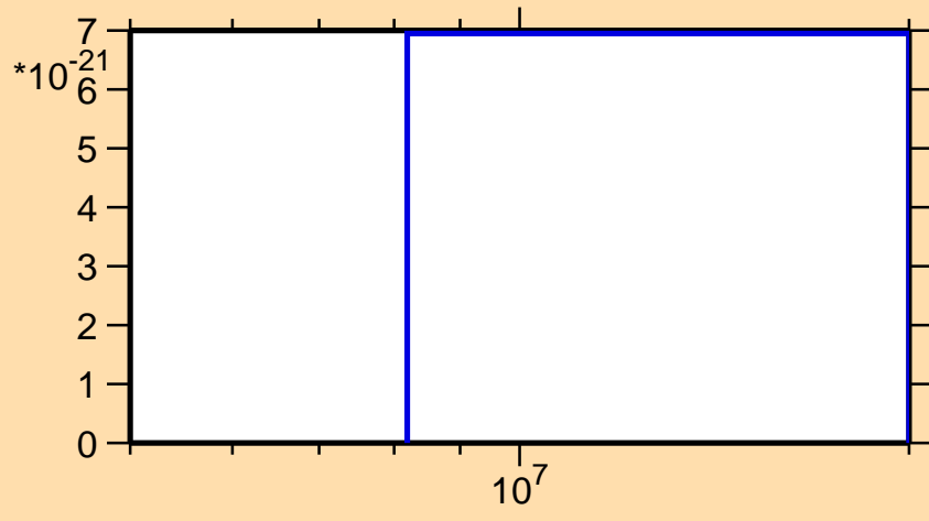
\sigma vs. E for ^{187}\text{Ta} (mt 42)
