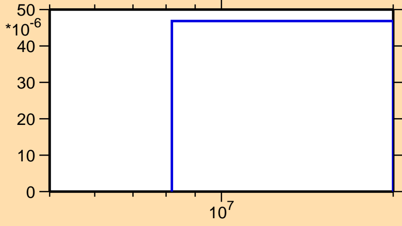
\sigma vs. E for ^{187}\text{Ta}(n,d)
