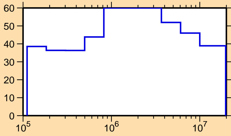
\Delta\sigma/\sigma vs. E for ^{188}\text{Ta}(n,n_1)
