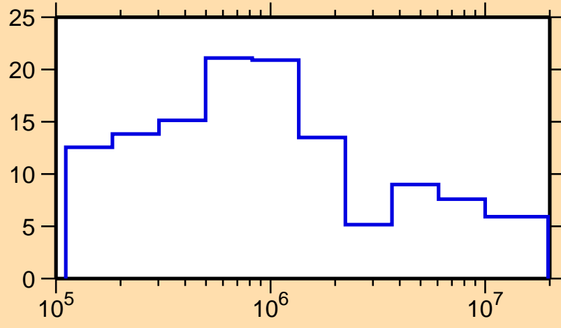
\Delta\sigma/\sigma vs. E for ^{188}\text{Ta}(n,tot.)
