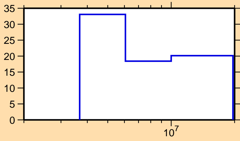
\Delta\sigma/\sigma vs. E for ^{188}\text{Ta}(n,2n)
