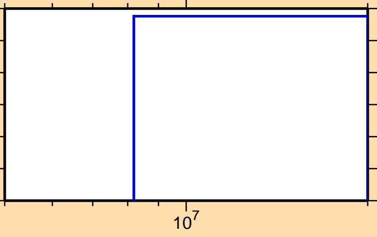
\sigma vs. E for ^{188}\text{Ta}(n,n\alpha)
