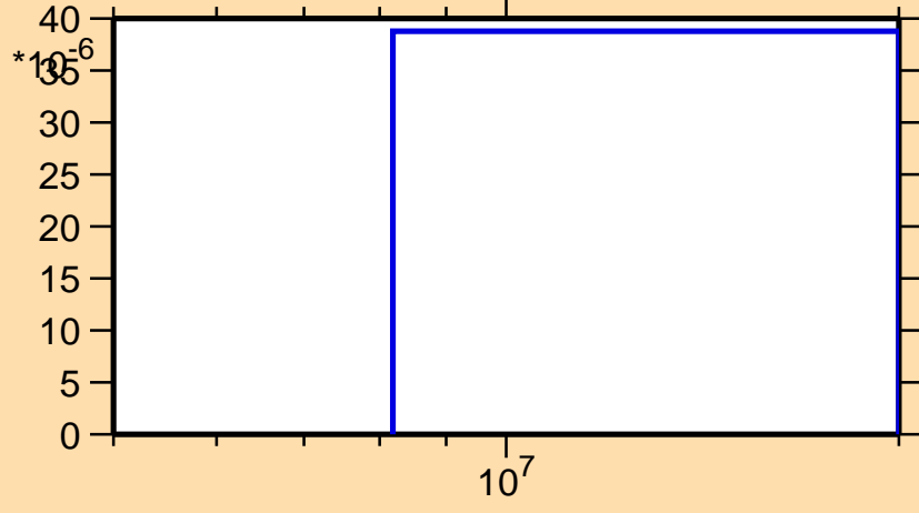
\sigma vs. E for ^{188}\text{Ta}(n,d)
