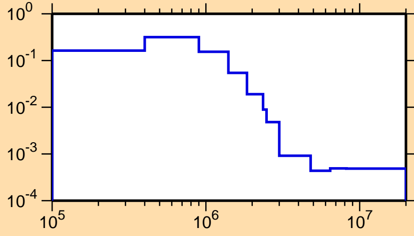
\sigma vs. E for ^{188}\text{Ta}(n,n_1)
