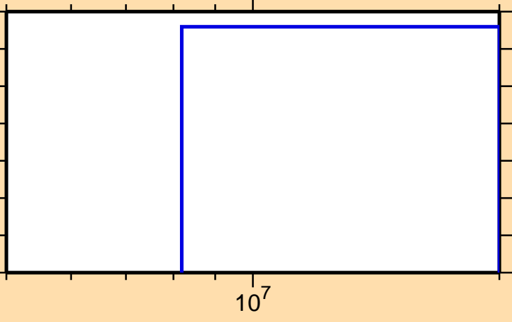
\sigma vs. E for ^{188}\text{Ta} (mt 42)
