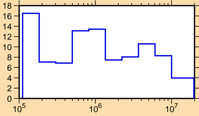
\Delta\sigma/\sigma vs. E for ^{189}\text{Ta}(n,tot.)
