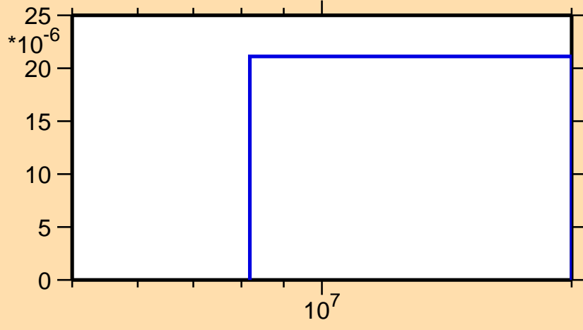
\sigma vs. E for ^{189}\text{Ta}(n,d)
