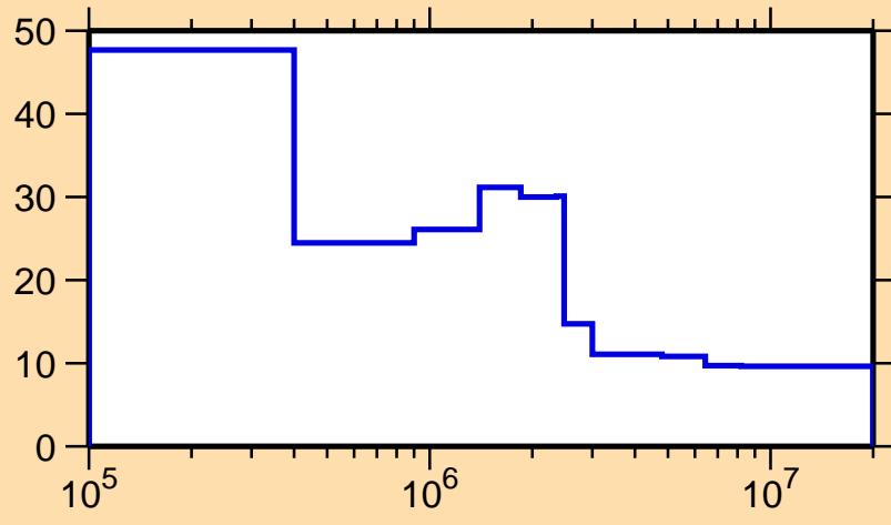
\Delta\sigma/\sigma vs. E for ^{189}\text{Ta}(n,\text{nonel.})
