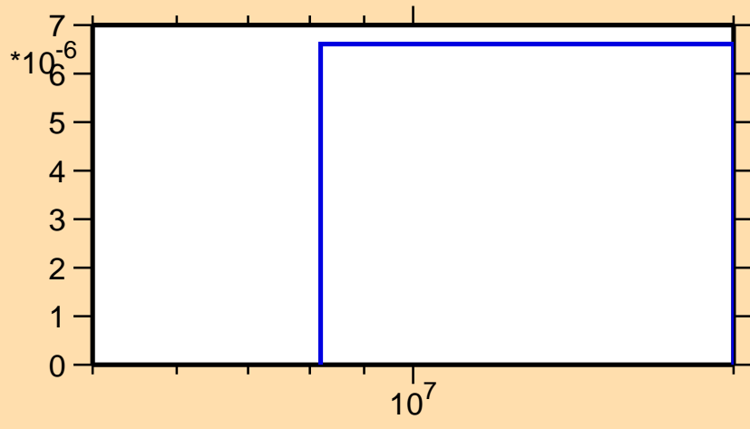
\sigma vs. E for ^{189}\text{Ta}(n,t)
