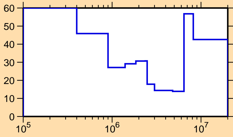
\Delta\sigma/\sigma vs. E for ^{189}\text{Ta}(n,n\text{cont.})
