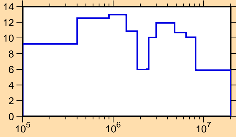
\Delta\sigma/\sigma vs. E for ^{190}\text{Ta}(n,tot.)
