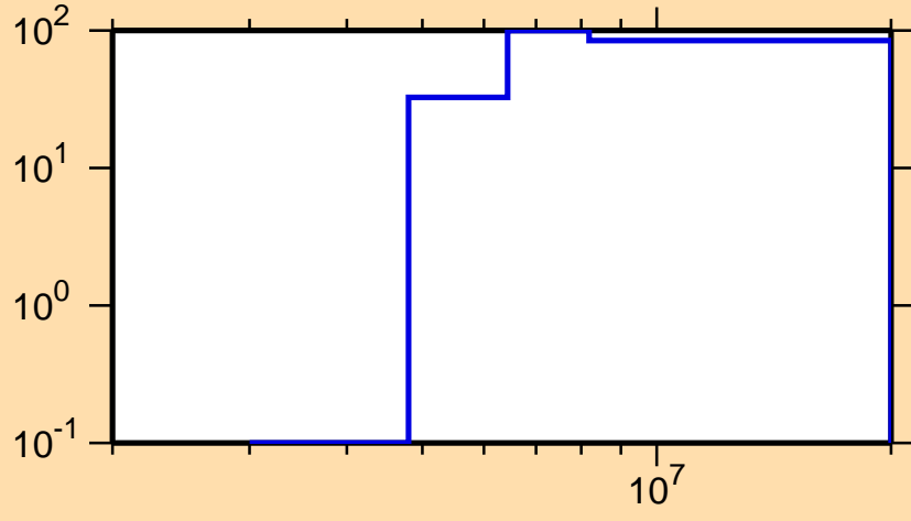
\Delta\sigma/\sigma vs. E for ^{190}\text{Ta}(n,p)
