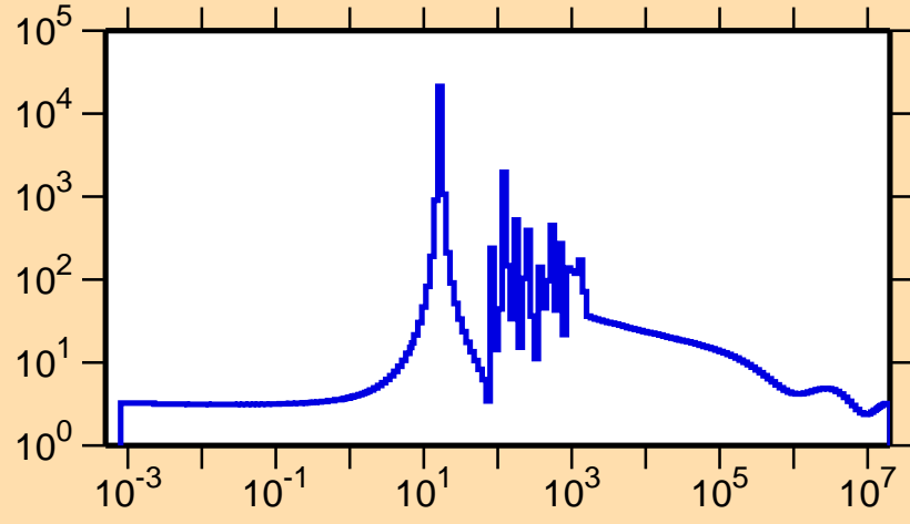
\sigma vs. E for ^{191}\text{Ta}(n,\text{el.})
