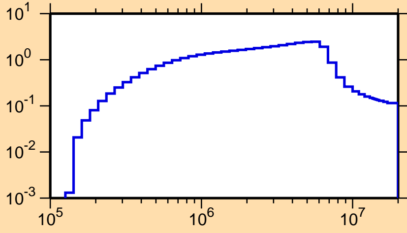
\sigma vs. E for ^{191}\text{Ta}(n,n\text{cont.})
