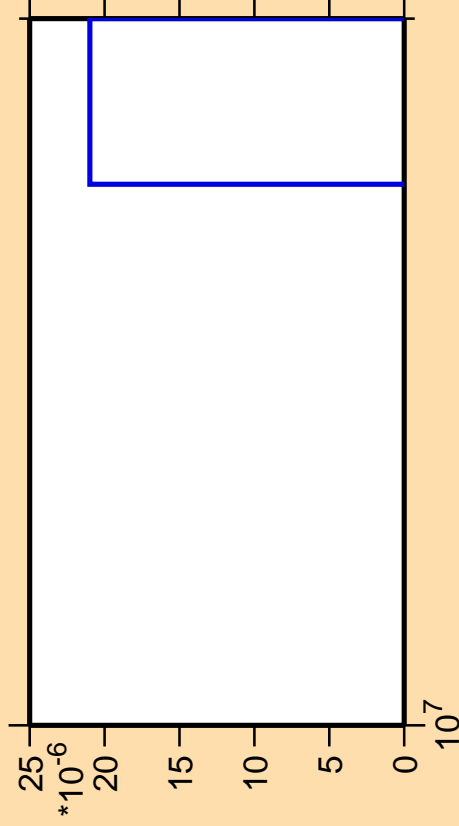
\Delta\sigma/\sigma vs. E for ^{191}\text{Ta} (mt 42)
