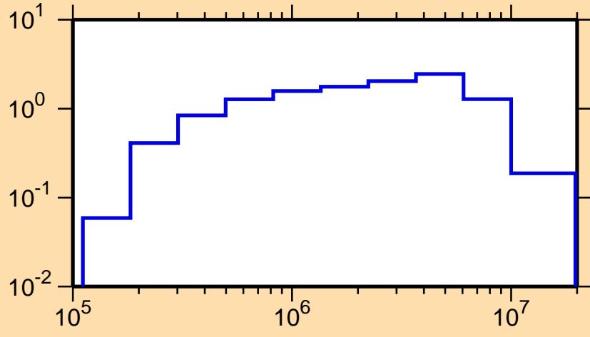
\sigma vs. E for ^{191}\text{Ta}(n,\text{inel.})
