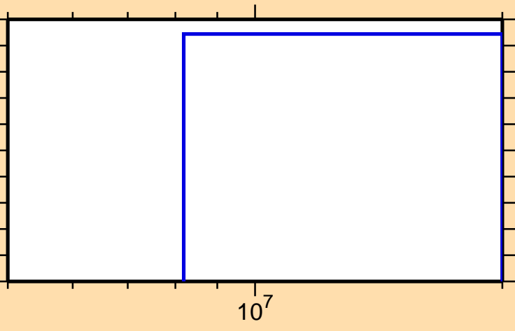
\sigma vs. E for ^{191}\text{Ta}(n,nt)
