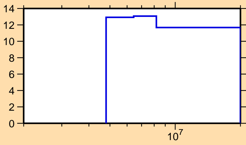
\Delta\sigma/\sigma vs. E for ^{191}\text{Ta}(n,\text{nonel.})
