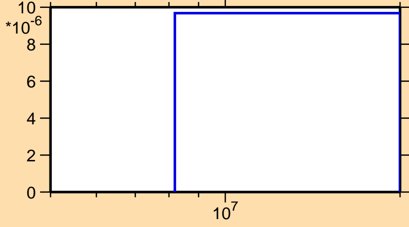
\sigma vs. E for ^{191}\text{Ta}(n,d)
