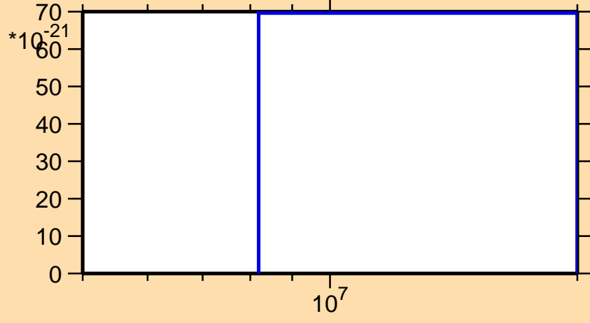
\sigma vs. E for ^{191}\text{Ta} (mt 42)
