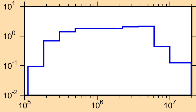
\sigma vs. E for ^{192}\text{Ta}(n,n\text{cont.})
