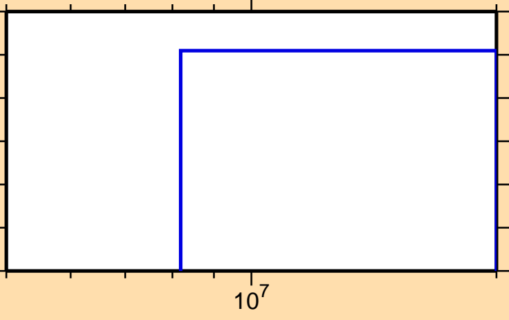
\sigma vs. E for ^{192}\text{Ta}(n,t)
