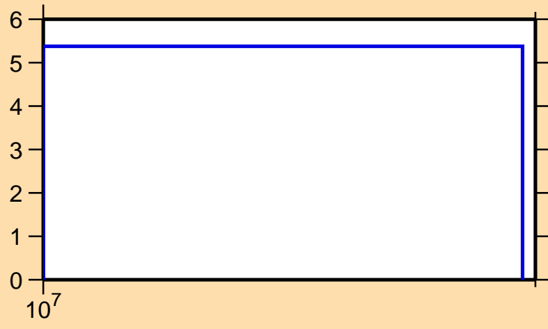
\Delta\sigma/\sigma vs. E for ^{139}\text{Tb}(n,\text{el.})
