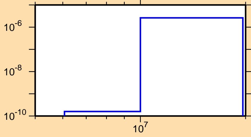
\sigma vs. E for ^{139}\text{Tb}(\text{mt117})
