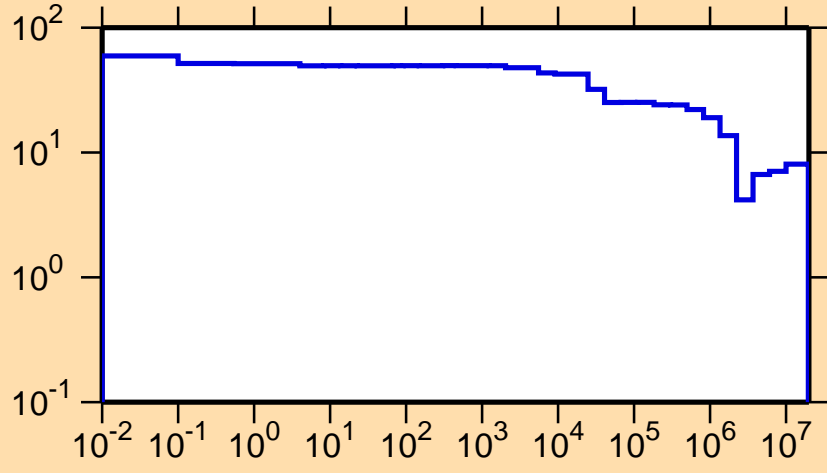
\Delta\sigma/\sigma vs. E for ^{139}\text{Tb}(n,\text{nonel.})
