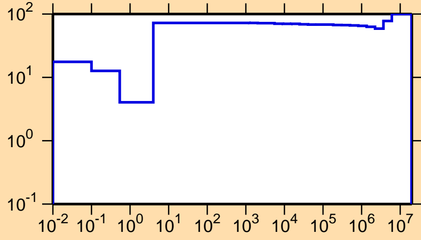
\Delta\sigma/\sigma vs. E for ^{139}\text{Tb}(n,\gamma)
