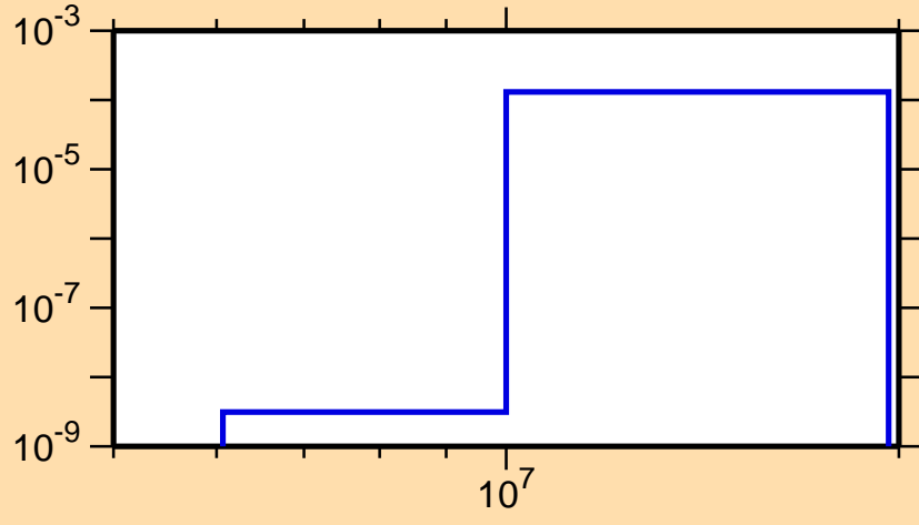
\sigma vs. E for ^{139}\text{Tb}(\text{mt } 45)
