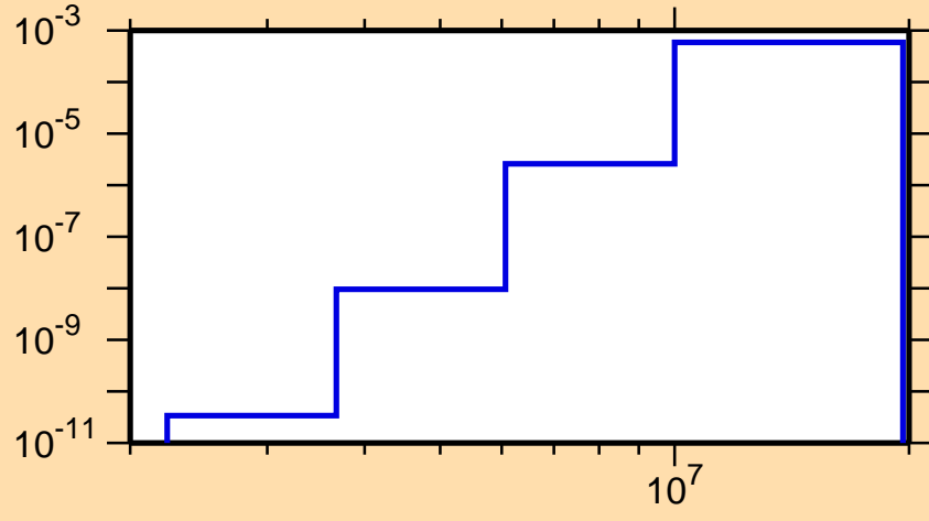
\sigma vs. E for ^{139}\text{Tb}(n,n\alpha)
