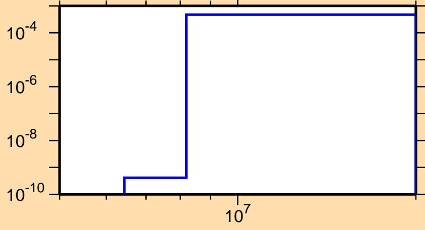
\sigma vs. E for ^{139}\text{Tb}(n,\text{pd})
