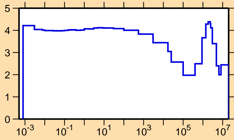
\sigma vs. E for ^{139}\text{Tb}(n,\text{el.})
