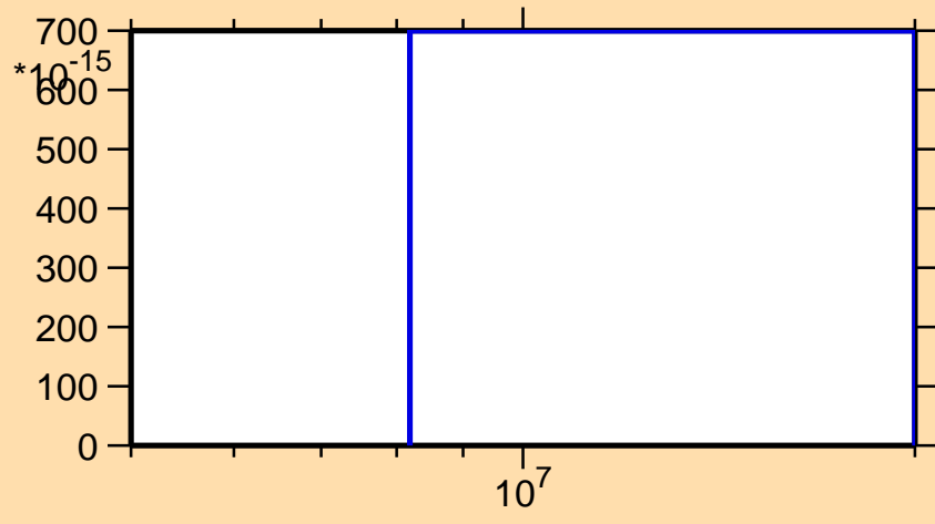
\sigma vs. E for ^{139}\text{Tb}(n,2n\alpha)
