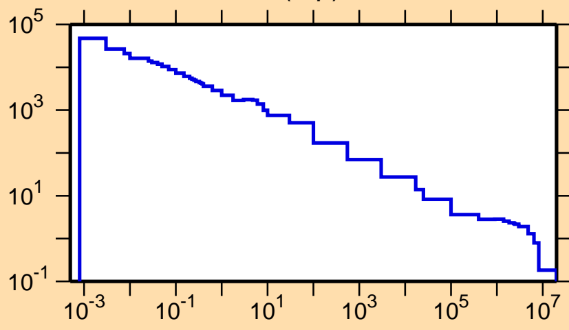
\sigma vs. E for ^{139}\text{Tb}(n,p)
