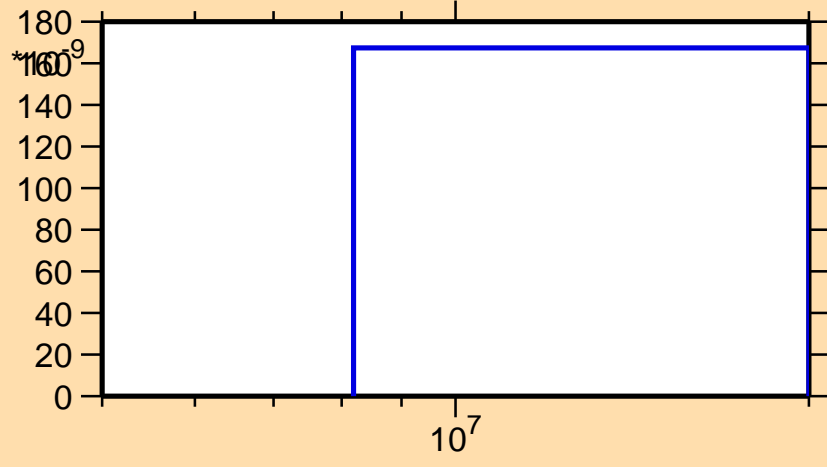
\sigma vs. E for ^{139}\text{Tb}(n,\text{pt})
