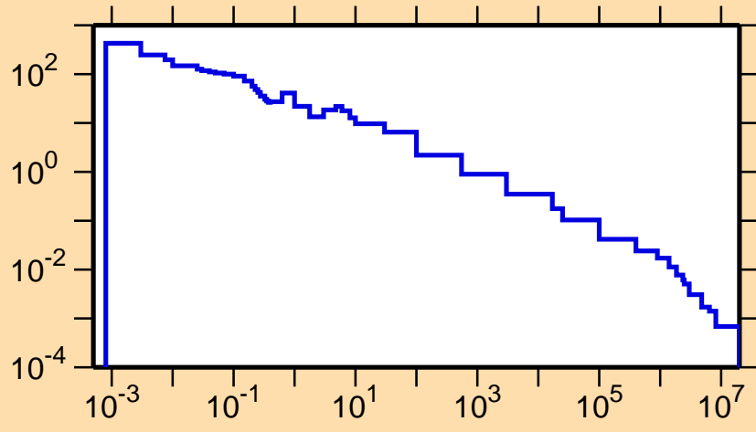
\sigma vs. E for ^{139}\text{Tb}(n,\gamma)
