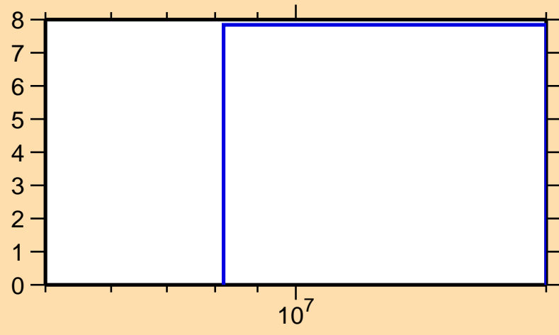
\Delta\sigma/\sigma vs. E for ^{139}\text{Tb}(n,\text{nonel.})
