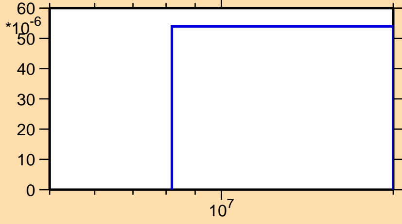
\sigma vs. E for ^{139}\text{Tb}(n,2n)
