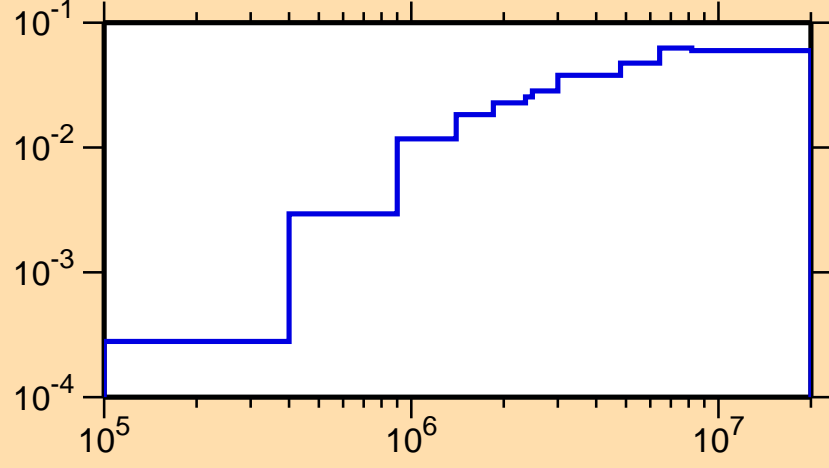
\sigma vs. E for ^{139}\text{Tb}(n,n\text{cont.})
