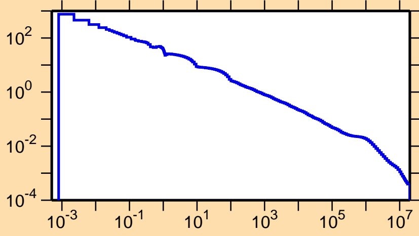
\sigma vs. E for ^{140}\text{Tb}(n,\gamma)
