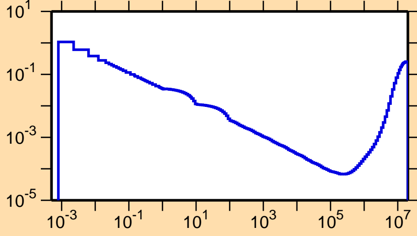
\sigma vs. E for ^{140}\text{Tb}(n,p\alpha)
