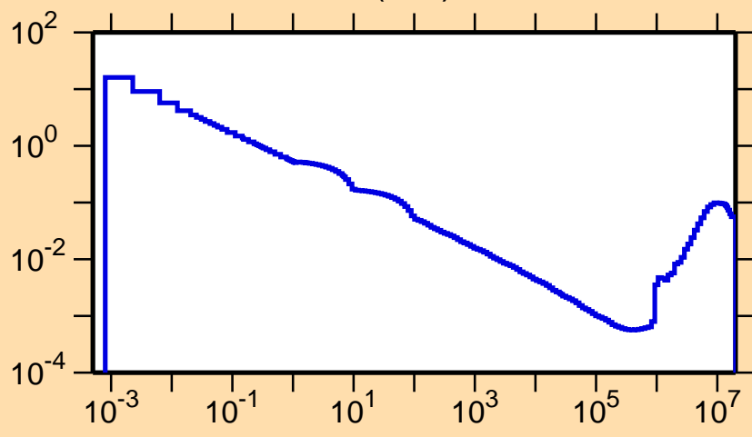
\sigma vs. E for ^{140}\text{Tb}(n,\alpha)
