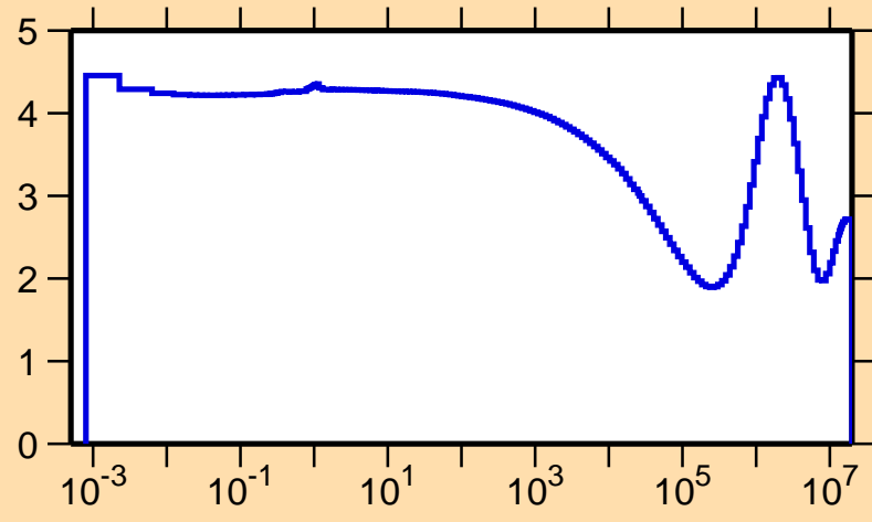
\sigma vs. E for ^{140}\text{Tb}(n,\text{el.})
