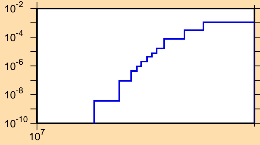
\sigma vs. E for ^{140}\text{Tb}(n,2np)
