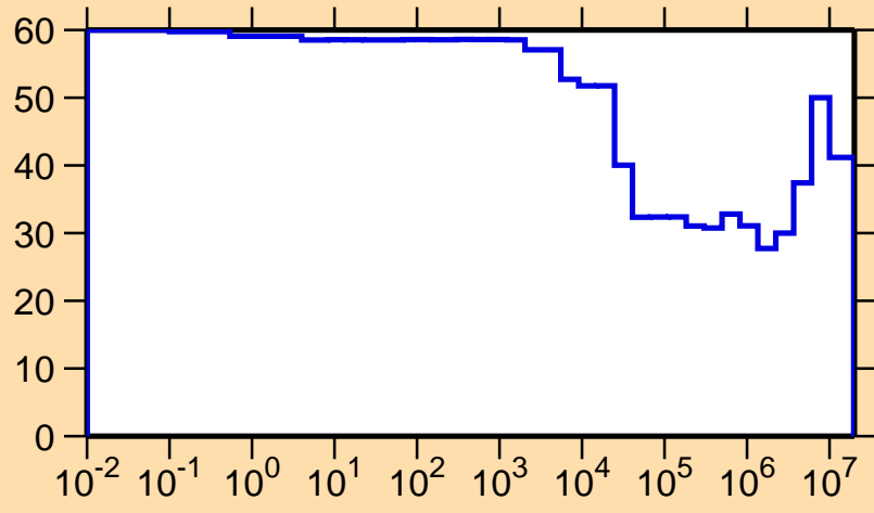
\Delta\sigma/\sigma vs. E for ^{140}\text{Tb}(n,p)
