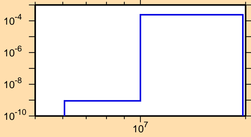
\sigma vs. E for ^{140}\text{Tb}(n,\text{pd})
