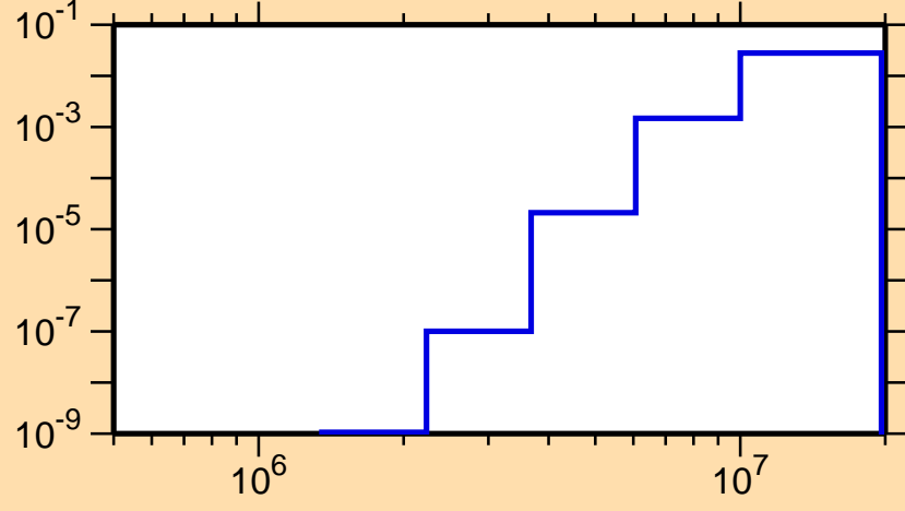
\sigma vs. E for ^{140}\text{Tb}(n,d)
