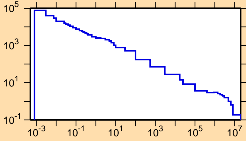
\sigma vs. E for ^{140}\text{Tb}(n,p)
