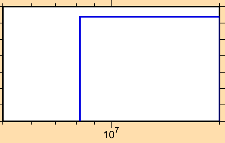
\sigma vs. E for ^{140}\text{Tb}(n,2np)
