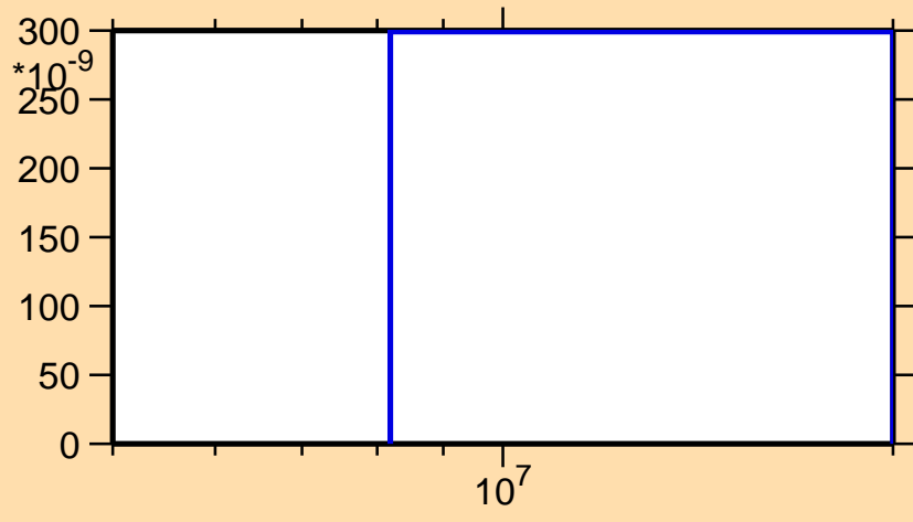
\sigma vs. E for ^{140}\text{Tb}(n,\text{nd})
