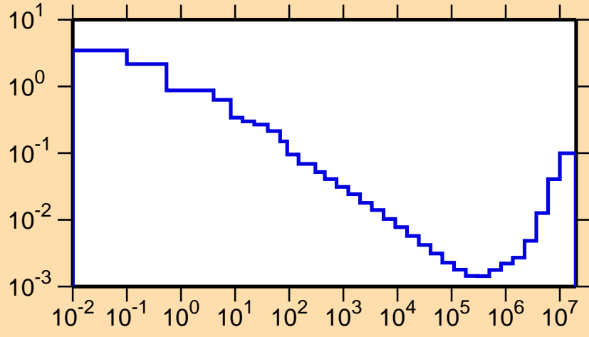
\sigma vs. E for ^{141}\text{Tb}(n,\alpha)
