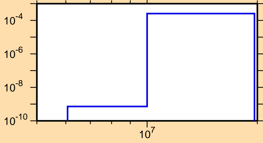
\sigma vs. E for ^{141}\text{Tb}(n,\text{pd})
