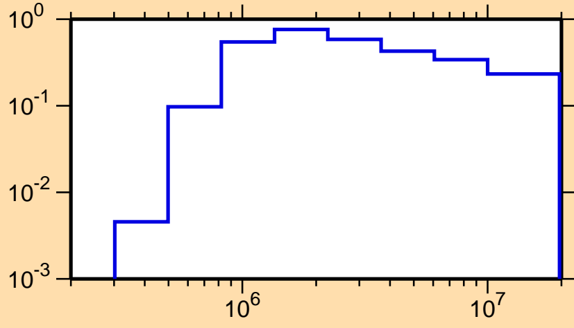
\sigma vs. E for ^{141}\text{Tb}(n,\text{inel.})
