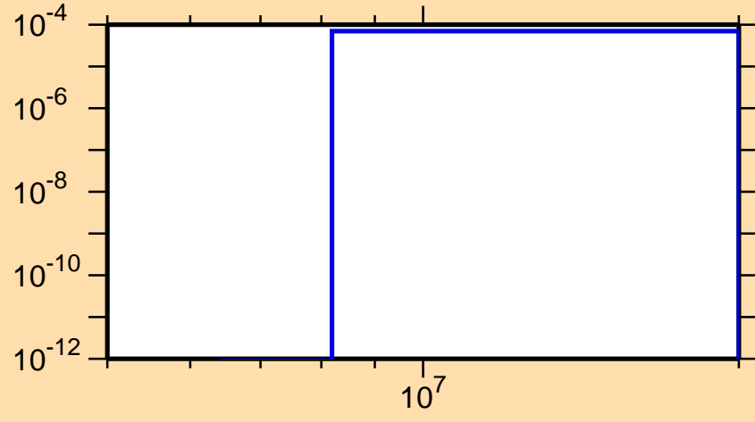
\sigma vs. E for ^{141}\text{Tb} (mt 45)
