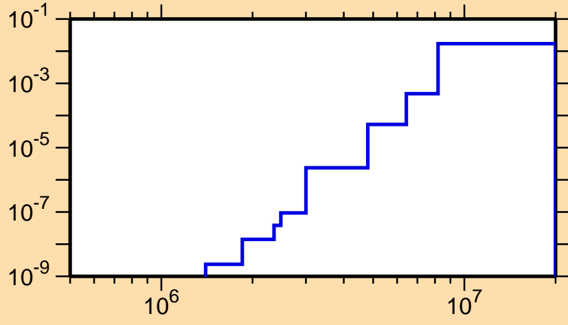
\sigma vs. E for ^{141}\text{Tb}(n,d)
