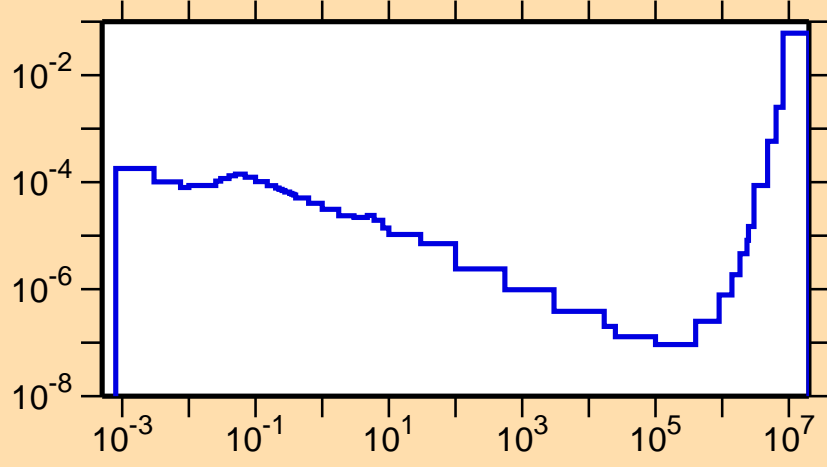
\sigma vs. E for ^{141}\text{Tb}(n,p\alpha)
