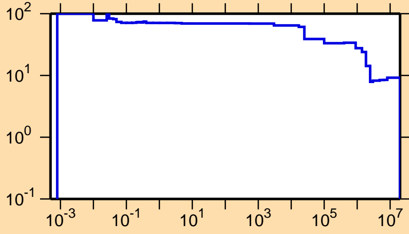
\Delta\sigma/\sigma vs. E for ^{141}\text{Tb}(n,\text{nonel.})
