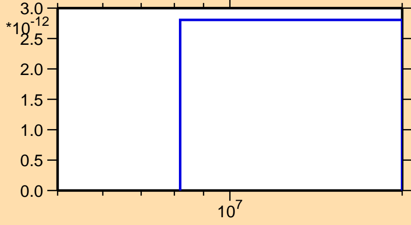
\sigma vs. E for ^{141}\text{Tb}(n,2n\alpha)
