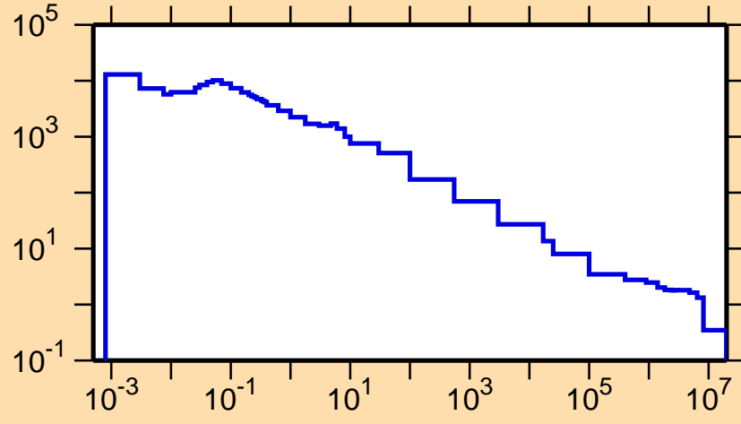
\sigma vs. E for ^{141}\text{Tb}(n,p)
