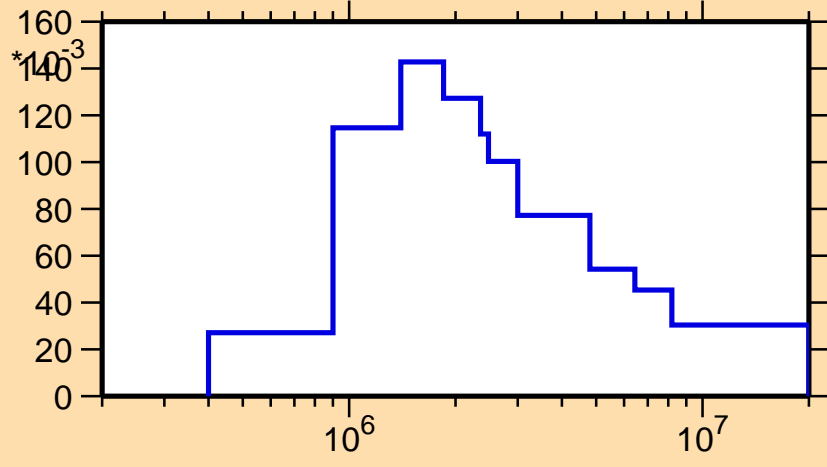
\sigma vs. E for ^{141}\text{Tb}(n,n_2)
