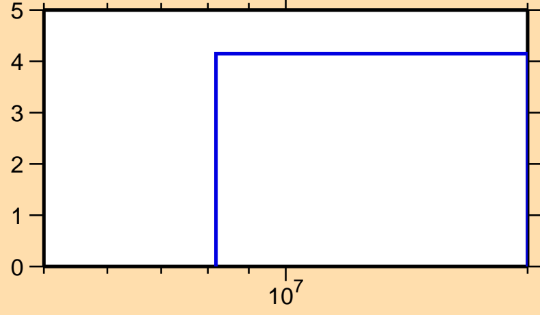
\Delta\sigma/\sigma vs. E for ^{141}\text{Tb}(n,\text{tot.})
