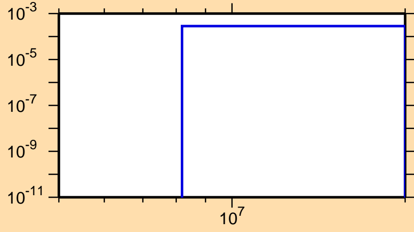
\sigma vs. E for ^{141}\text{Tb}(n,pd)
