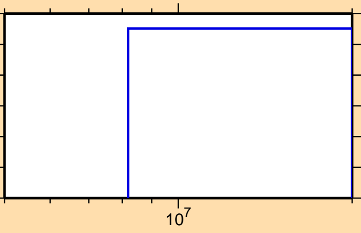
\sigma vs. E for ^{141}\text{Tb}(n,2n\alpha)
