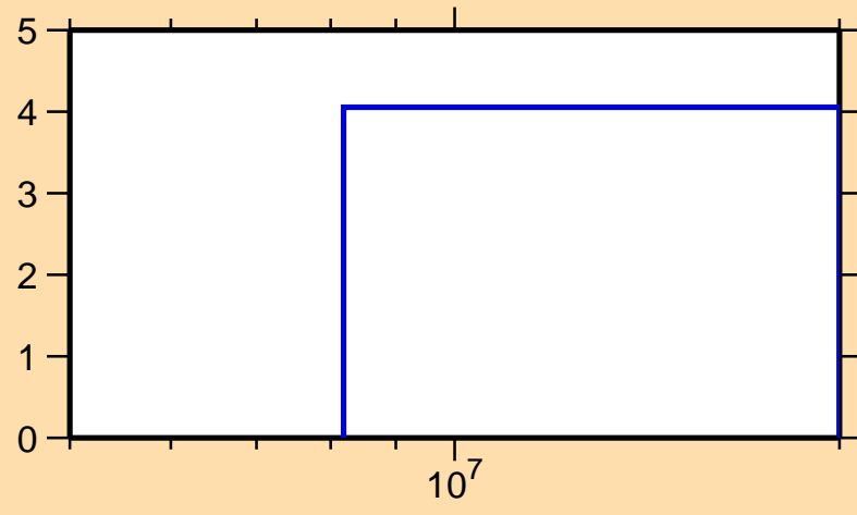
\Delta\sigma/\sigma vs. E for ^{143}\text{Tb}(n,\text{tot.})
