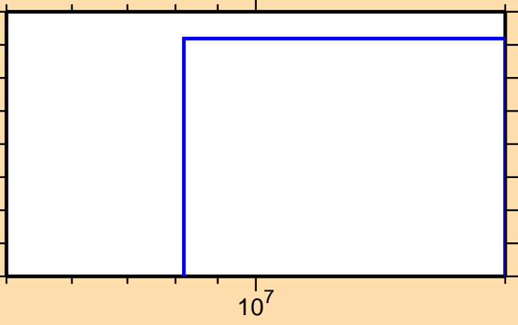
\sigma vs. E for ^{143}\text{Tb}(n,2n\alpha)
