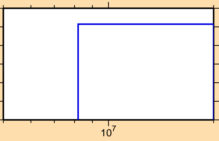
\sigma vs. E for ^{143}\text{Tb}(n,\text{pd})
