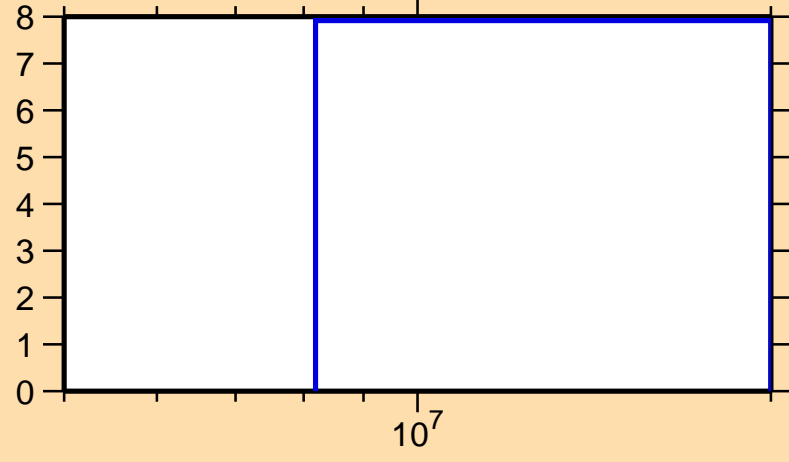
\Delta\sigma/\sigma vs. E for ^{143}\text{Tb}(n,\text{el.})
