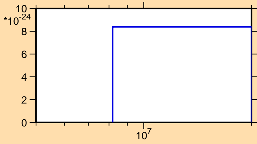
\sigma vs. E for ^{143}\text{Tb}(\text{mt } 11)
