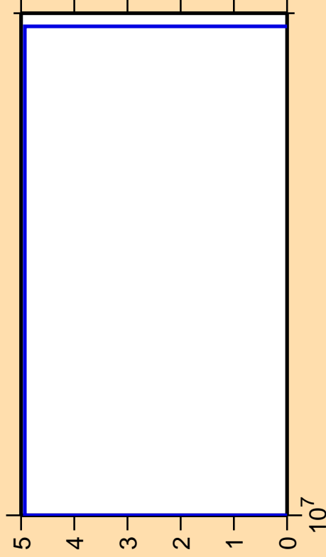
\Delta\sigma/\sigma vs. E for ^{144}\text{Tb}(n,nt)
