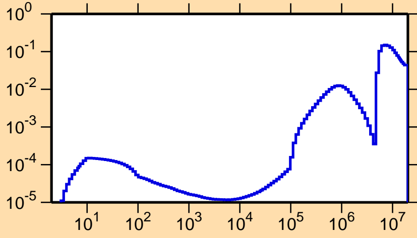
\sigma vs. E for ^{144}\text{Tb}(n,\text{inel.})
