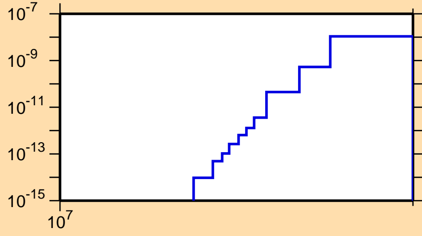
\sigma vs. E for ^{144}\text{Tb} (mt 34)
