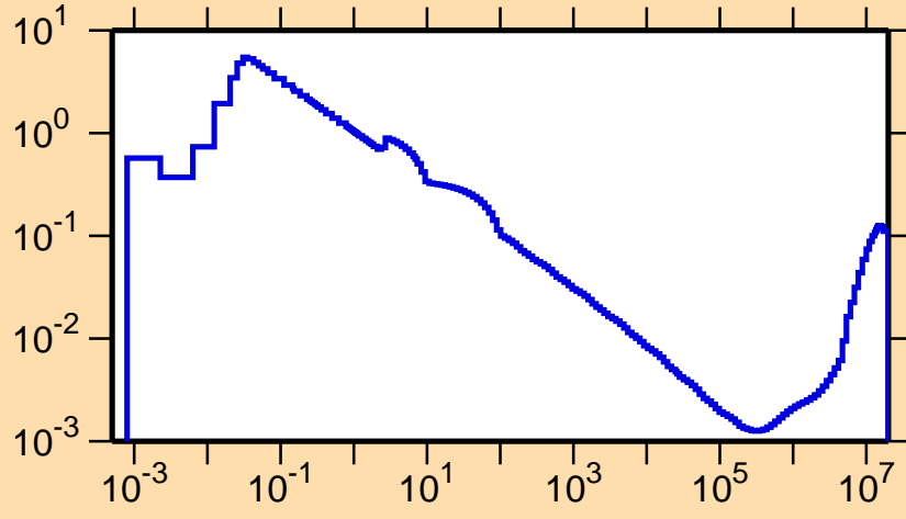
\sigma vs. E for ^{144}\text{Tb}(n,\alpha)
