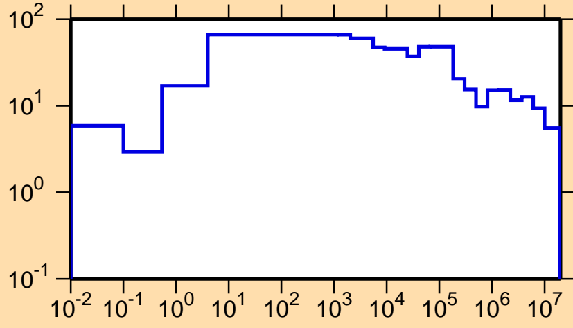
\Delta\sigma/\sigma vs. E for ^{144}\text{Tb}(n, tot.)
