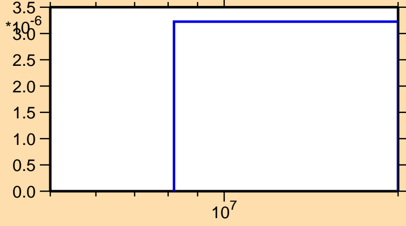
\sigma vs. E for ^{144}\text{Tb}(n,pd)
