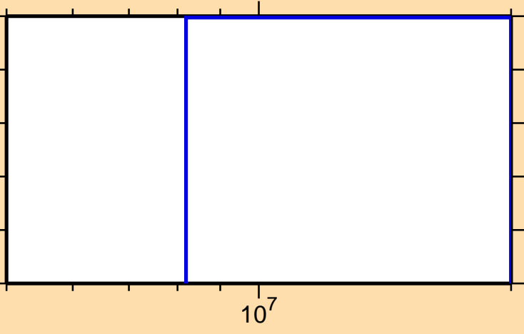
\sigma vs. E for ^{144}\text{Tb}(n,\text{nd})
