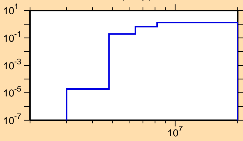
\sigma vs. E for ^{144}\text{Tb}(n,np)
