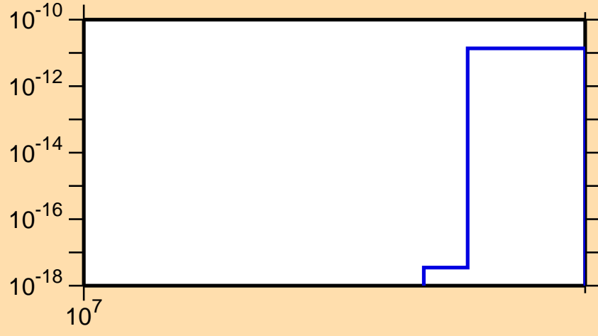
\sigma vs. E for ^{145}\text{Tb}(n,nt)
