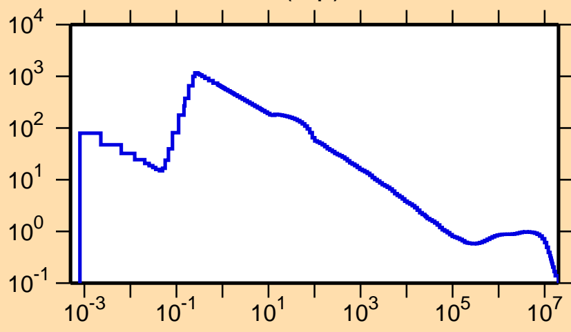
\sigma vs. E for ^{145}\text{Tb}(n,p)
