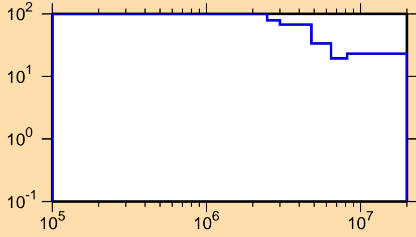
\Delta\sigma/\sigma vs. E for ^{145}\text{Tb}(n,\text{inel.})
