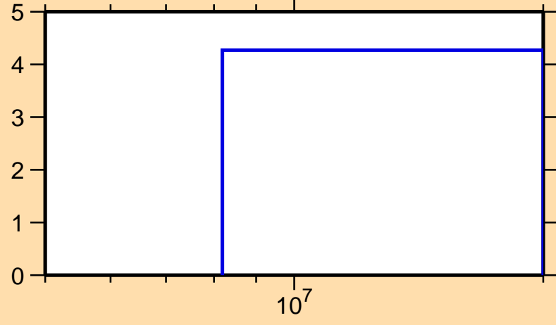
\Delta\sigma/\sigma vs. E for ^{145}\text{Tb}(n,\text{tot.})
