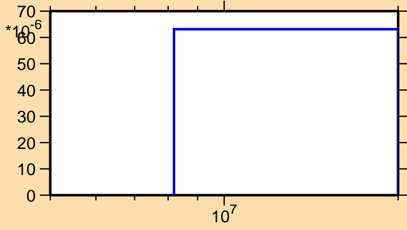
\sigma vs. E for ^{145}\text{Tb}(n,t)
