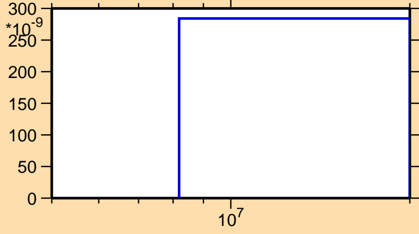
\sigma vs. E for ^{145}\text{Tb}(n,pd)
