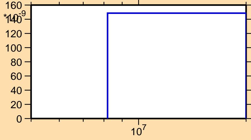
\sigma vs. E for ^{145}\text{Tb} (mt 45)
