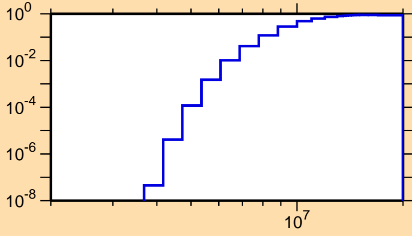
\sigma vs. E for ^{146}\text{Tb}(n,np)
