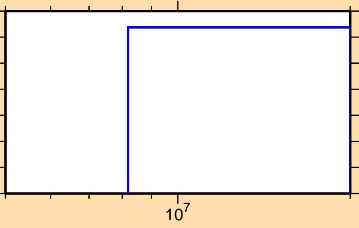
\sigma vs. E for ^{146}\text{Tb}(n,\text{nd})
