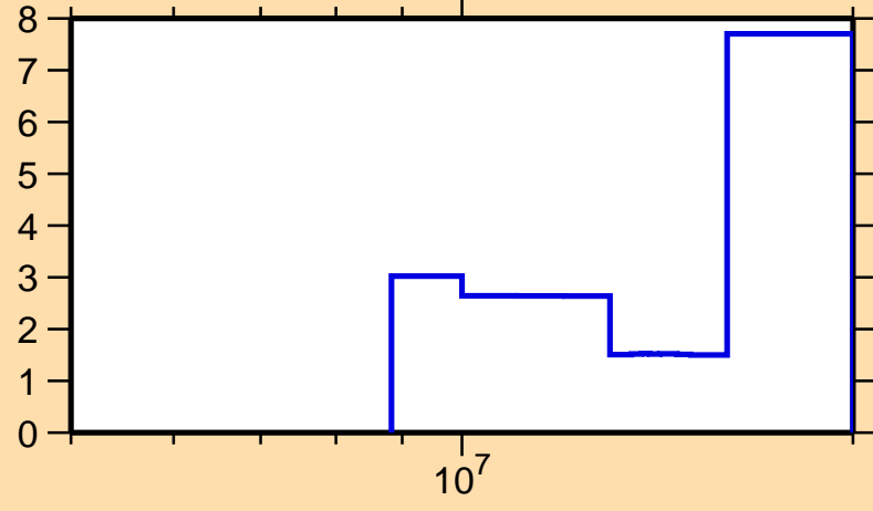
\Delta\sigma/\sigma vs. E for ^{146}\text{Tb}(n,\text{tot.})
