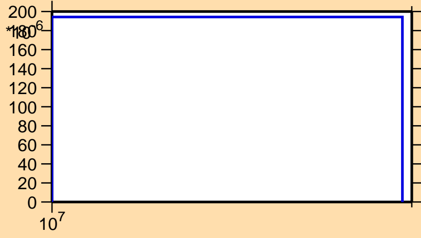
\sigma vs. E for ^{146}\text{Tb}(n,2np)
