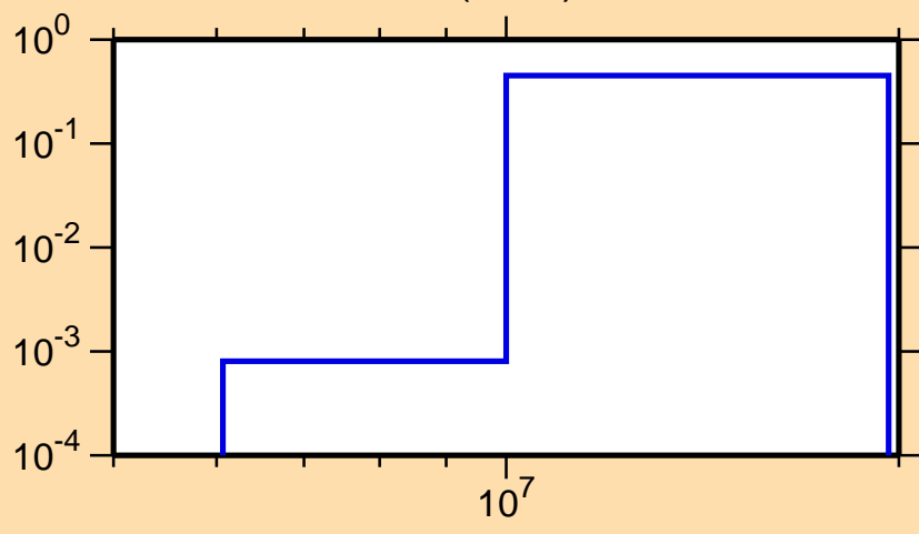
\sigma vs. E for ^{146}\text{Tb}(n,2n)
