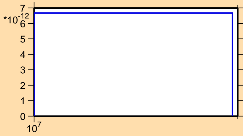
\sigma vs. E for ^{146}\text{Tb} (mt 34)
