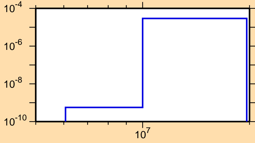
\sigma vs. E for ^{146}\text{Tb}(n,\text{He3})
