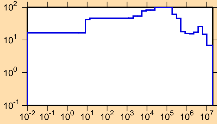
\Delta\sigma/\sigma vs. E for ^{146}\text{Tb}(n,\text{el.})
