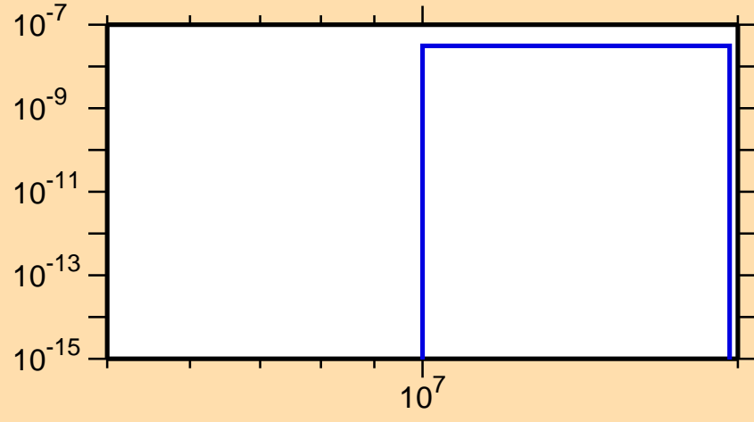
\sigma vs. E for ^{146}\text{Tb} (mt 45)
