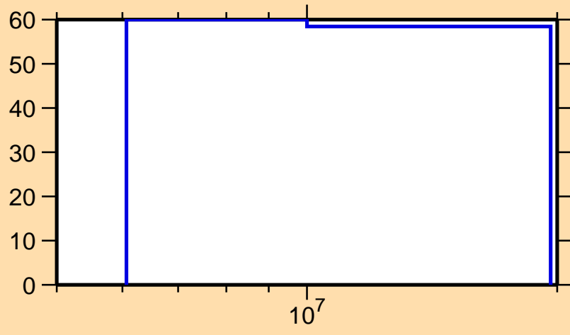
\Delta\sigma/\sigma vs. E for ^{146}\text{Tb}(n,2n)
