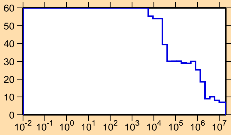
\Delta\sigma/\sigma vs. E for ^{146}\text{Tb}(n,\text{nonel.})
