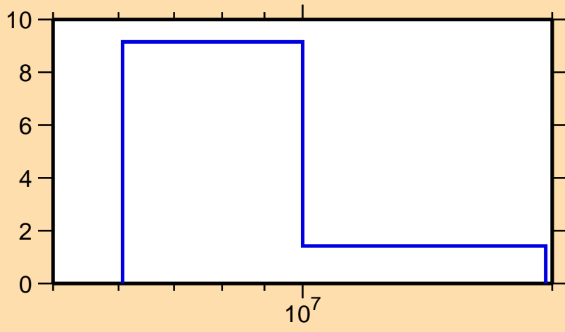
\Delta\sigma/\sigma vs. E for ^{146}\text{Tb}(n,\text{tot.})
