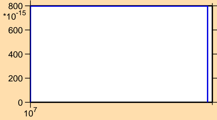
\sigma vs. E for ^{146}\text{Tb}(n,nt)
