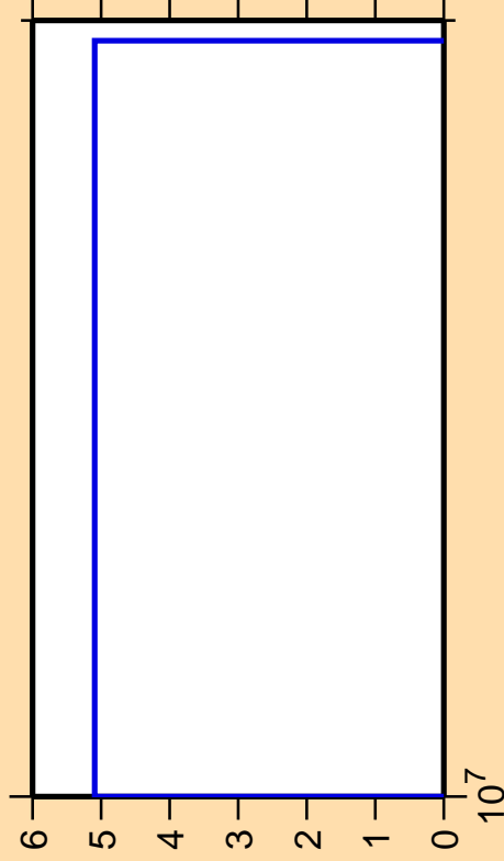
\Delta\sigma/\sigma vs. E for ^{146}\text{Tb}(n,nt)
