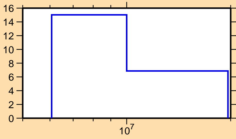
\Delta\sigma/\sigma vs. E for ^{146}\text{Tb}(n,\text{el.})
