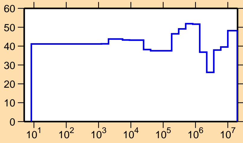
\Delta\sigma/\sigma vs. E for ^{146}\text{Tb}(n,n_1)
