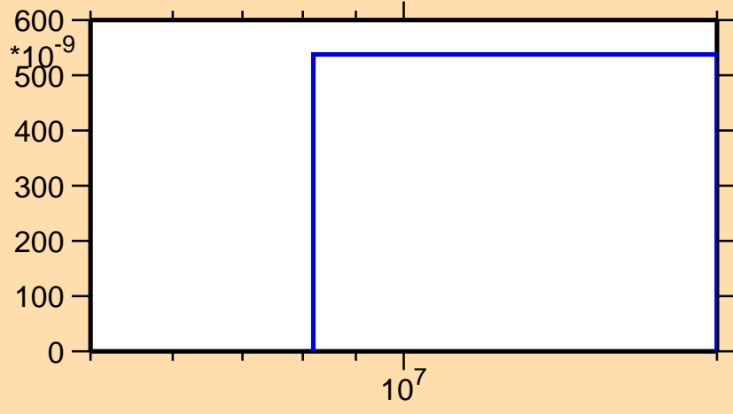
\sigma vs. E for ^{146}\text{Tb}(n,pd)
