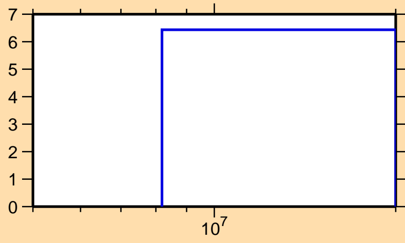
\Delta\sigma/\sigma vs. E for ^{146}\text{Tb}(n,\text{el.})
