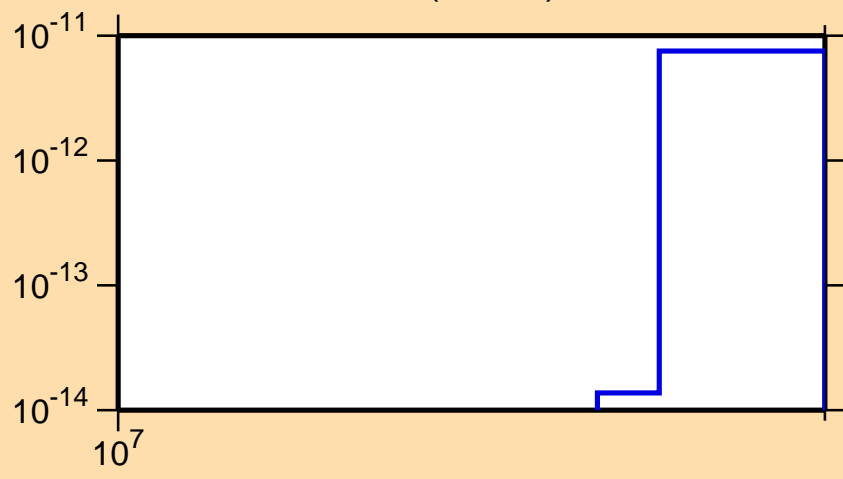
\sigma vs. E for ^{147}\text{Tb} (mt 34)
