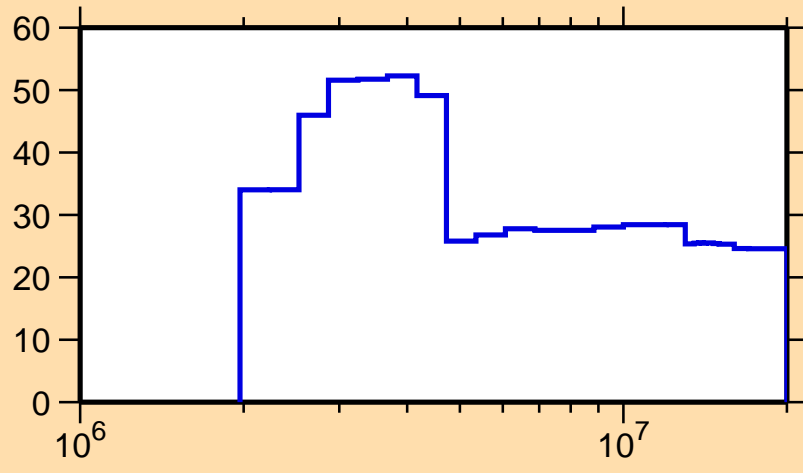
\Delta\sigma/\sigma vs. E for ^{147}\text{Tb}(n,n_1)
