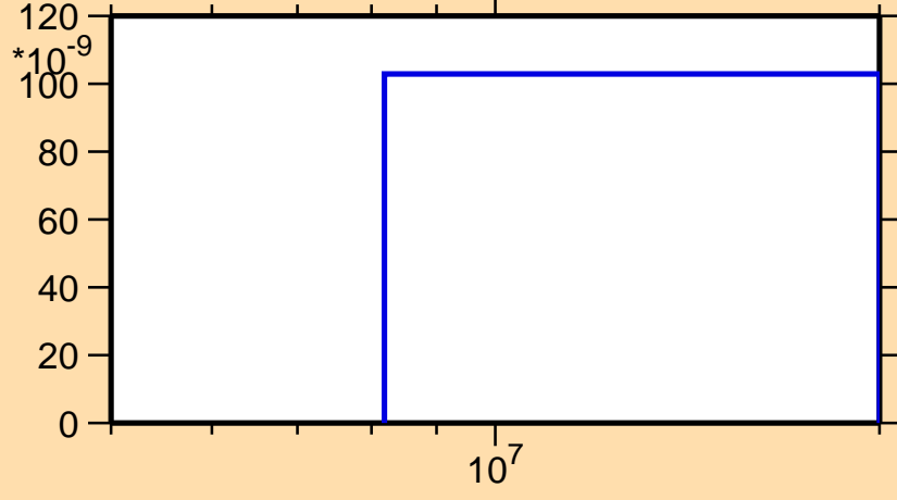
\sigma vs. E for ^{147}\text{Tb}(n,pd)
