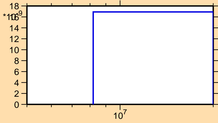
\sigma vs. E for ^{147}\text{Tb} (mt 45)
