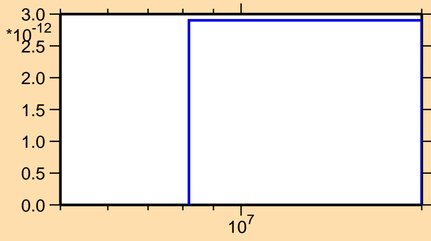
\sigma vs. E for ^{147}\text{Tb}(n,\text{pt})
