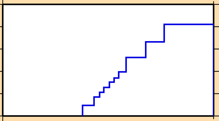
\sigma vs. E for ^{147}\text{Tb}(\text{mt117})
