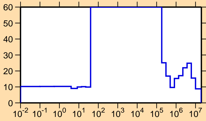
\Delta\sigma/\sigma vs. E for ^{147}\text{Tb}(n,el.)
