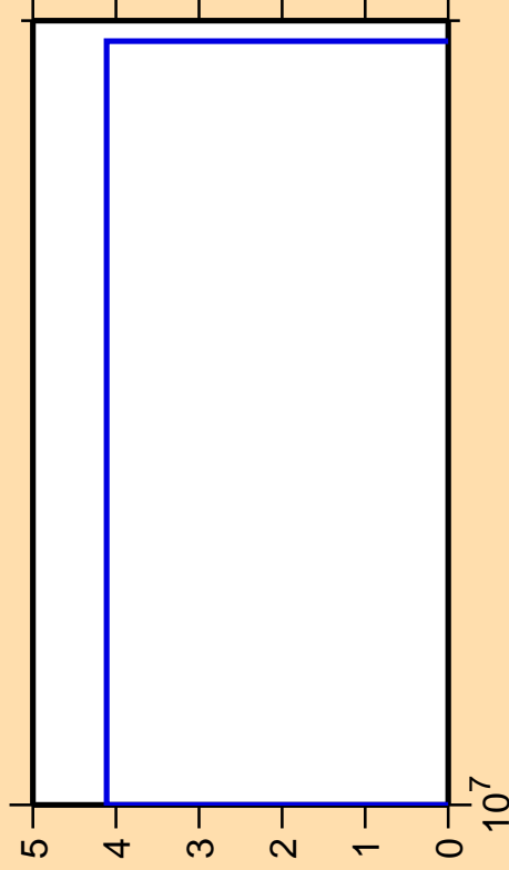
\Delta\sigma/\sigma vs. E for ^{147}\text{Tb}(n,2n\alpha)
