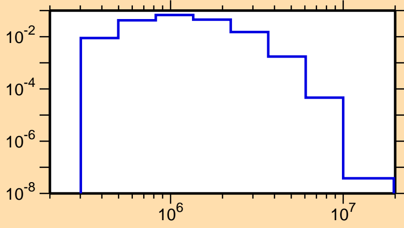
\sigma vs. E for ^{147}\text{Tb}(n,n_3)
