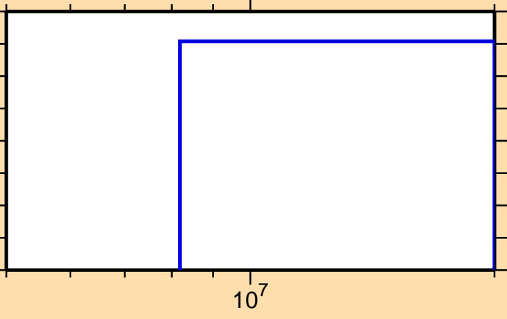
\sigma vs. E for ^{147}\text{Tb}(n,2n)
