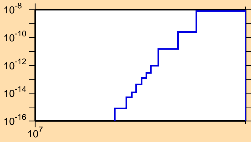
\sigma vs. E for ^{148}\text{Tb} (mt 34)
