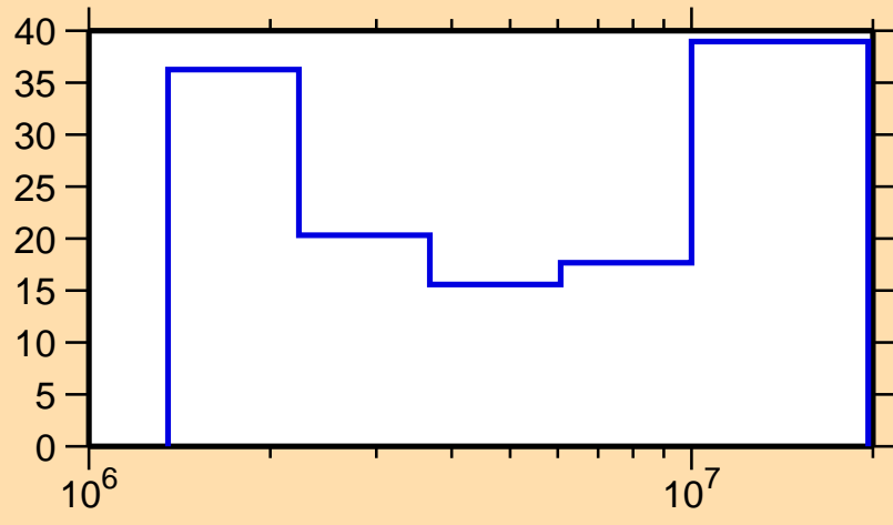
\Delta\sigma/\sigma vs. E for ^{148}\text{Tb}(n,n\text{cont.})
