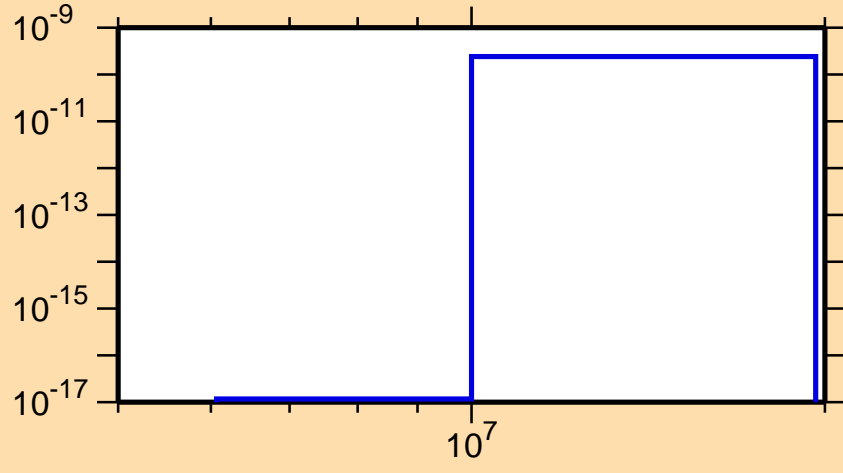
\sigma vs. E for ^{148}\text{Tb}(\text{mt117})
