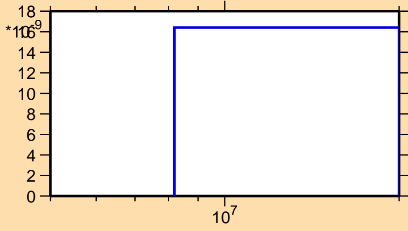
\sigma vs. E for ^{148}\text{Tb} (mt 45)
