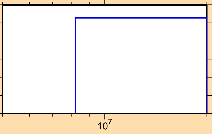
\sigma vs. E for ^{148}\text{Tb}(n,\text{pd})
