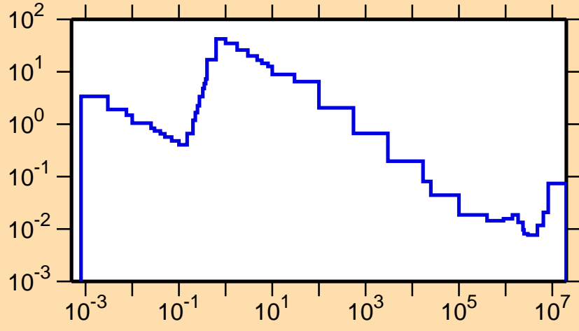
\sigma vs. E for ^{148}\text{Tb}(n,\alpha)
