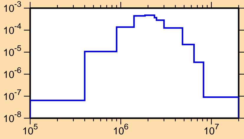
\sigma vs. E for ^{148}\text{Tb}(n,n_1)
