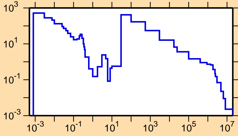
\sigma vs. E for ^{148}\text{Tb}(n,\gamma)
