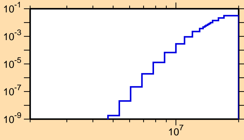
\sigma vs. E for ^{148}\text{Tb}(n,n\alpha)
