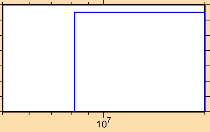
\sigma vs. E for ^{148}\text{Tb}(n,2n\alpha)
