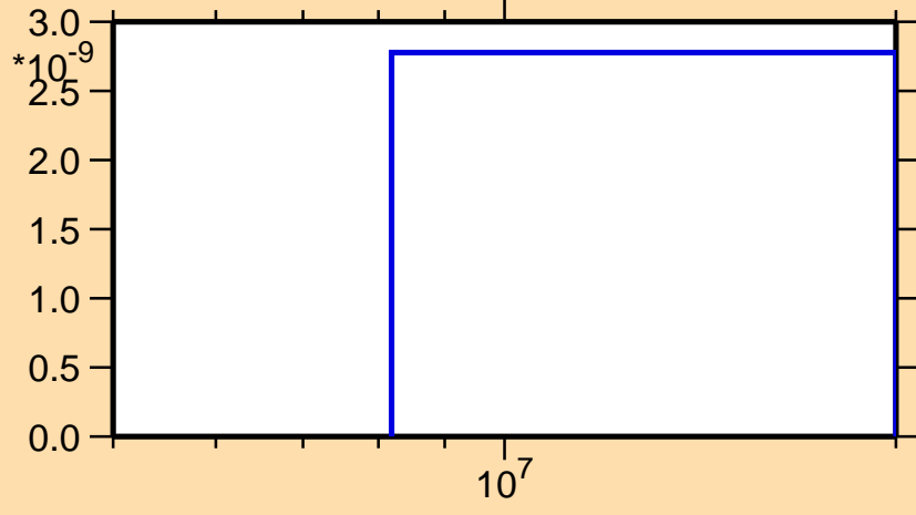
\sigma vs. E for ^{148}\text{Tb}(n,\text{pd})
