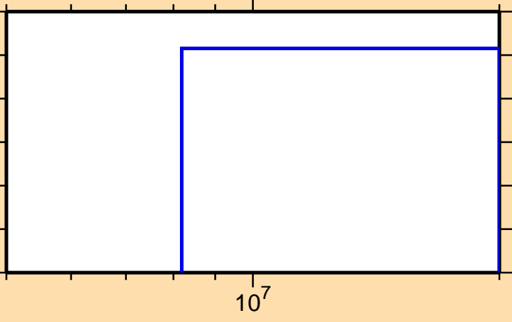
\sigma vs. E for ^{148}\text{Tb} (mt 45)
