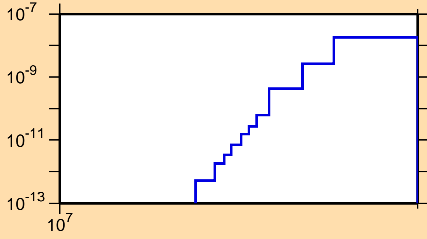
\sigma vs. E for ^{149}\text{Tb}(n,pd)
