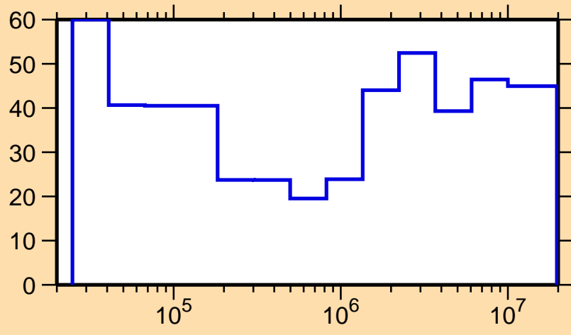
\Delta\sigma/\sigma vs. E for ^{149}\text{Tb}(n,n_1)
