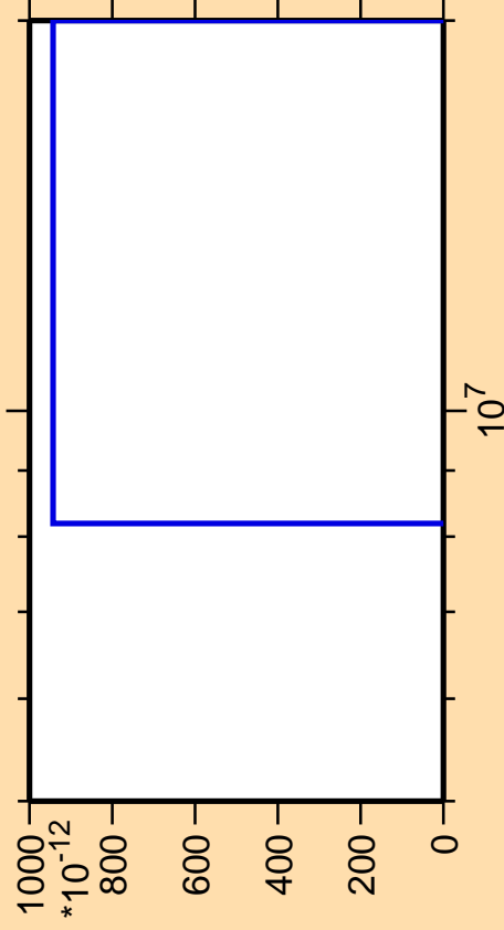
\Delta\sigma/\sigma vs. E for ^{150}\text{Tb}(\text{mt } 42)
