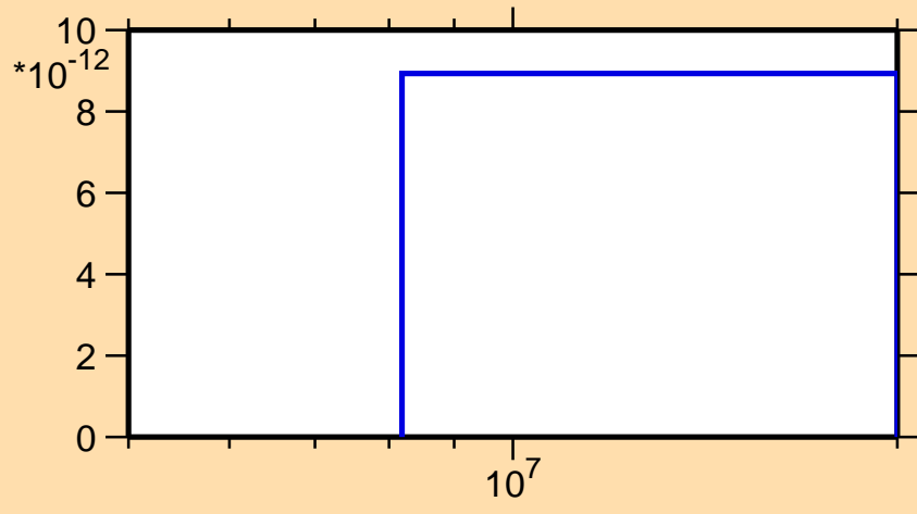
\sigma vs. E for ^{150}\text{Tb}(n,\text{pt})
