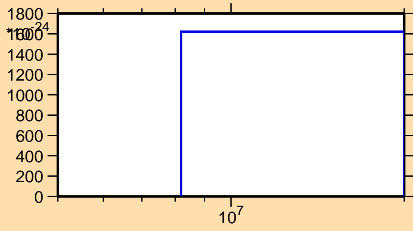
\sigma vs. E for ^{150}\text{Tb}(\text{mt } 42)
