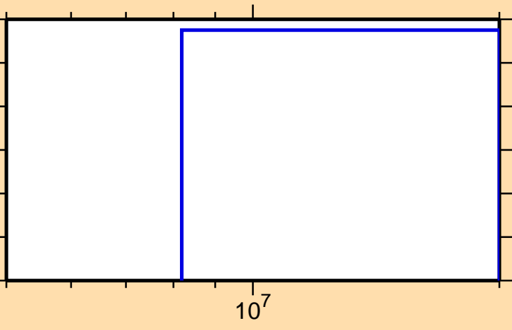
\sigma vs. E for ^{151}\text{Tb}(n,\text{He3})
