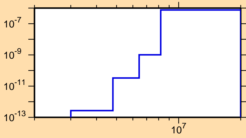
\sigma vs. E for ^{151}\text{Tb}(n,p\alpha)
