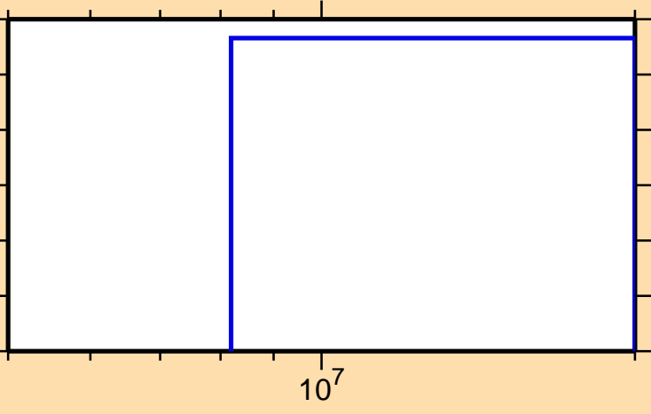
\sigma vs. E for ^{151}\text{Tb}(n,3n)
