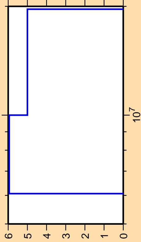
\Delta\sigma/\sigma vs. E for ^{151}\text{Tb}(n,2n)
