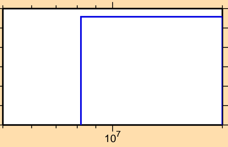
\sigma vs. E for ^{151}\text{Tb}(n,2np)
