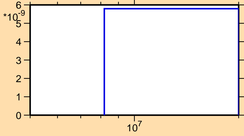
\sigma vs. E for ^{151}\text{Tb} (mt 45)
