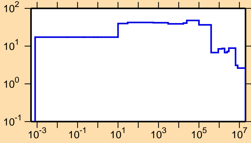
\Delta\sigma/\sigma vs. E for ^{151}\text{Tb}(n,el.)
